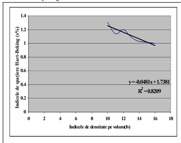
Fig. 3 Correlation between the Hart-Beking (s%) spacing factors and the values of density in volume (Iv) for the stands studied
